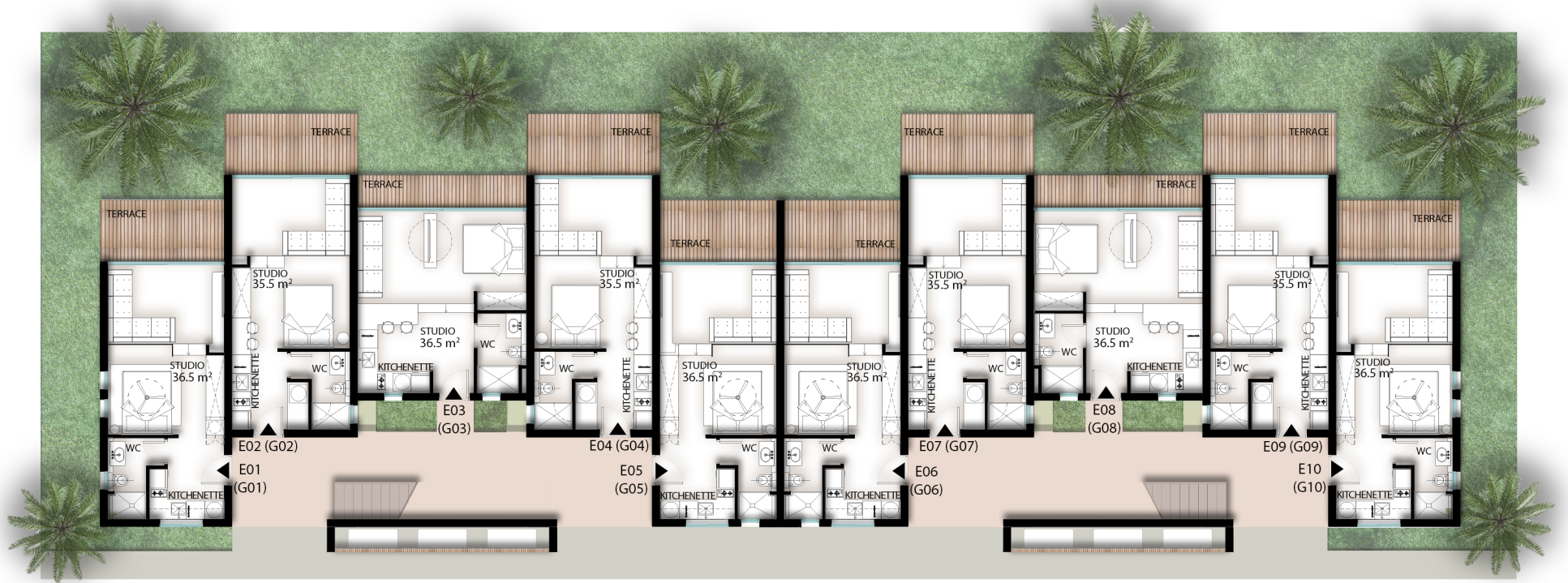
BLOCK E - GROUND FLOOR PLAN
