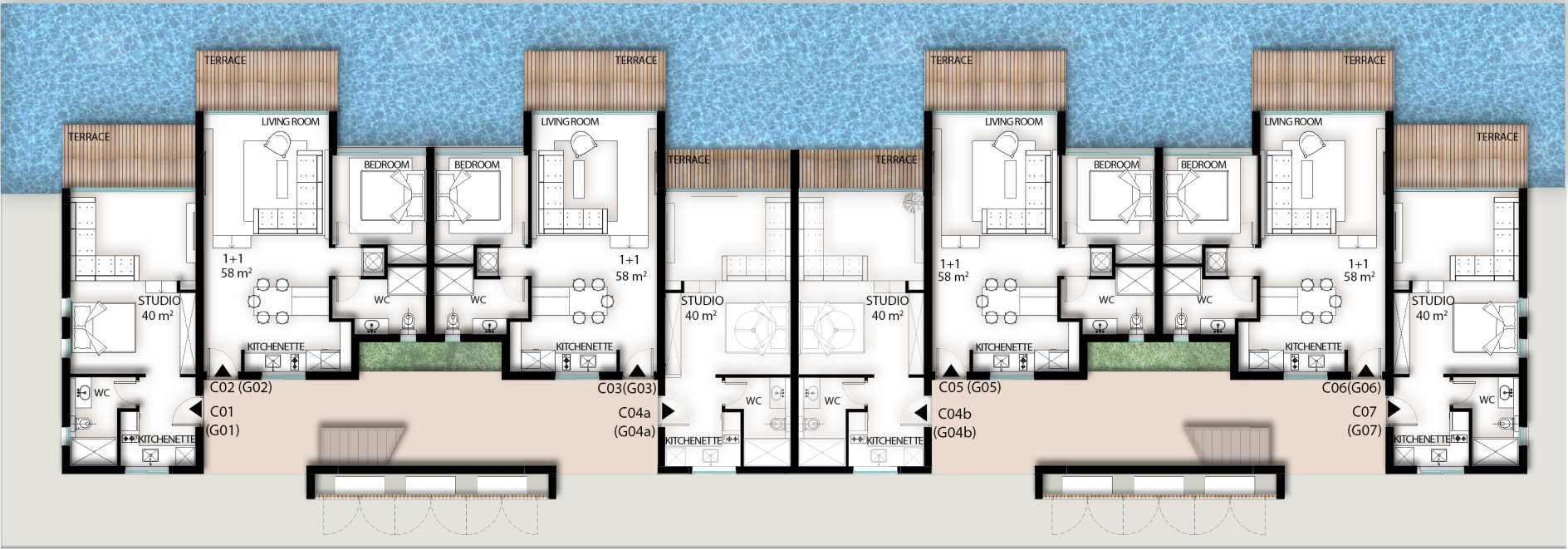
BLOCK C - GROUND FLOOR PLAN
