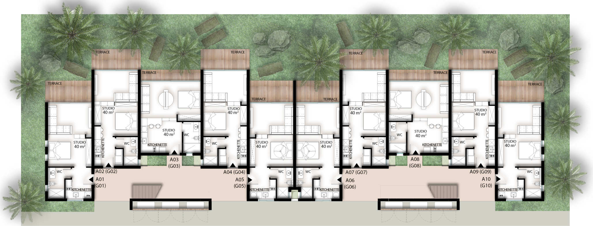
BLOCK A - GROUND FLOOR PLAN
